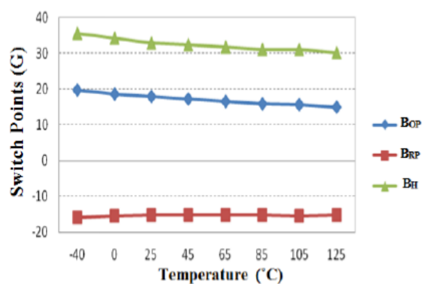
Temperature performance ( V_{CC}=3.0V )
