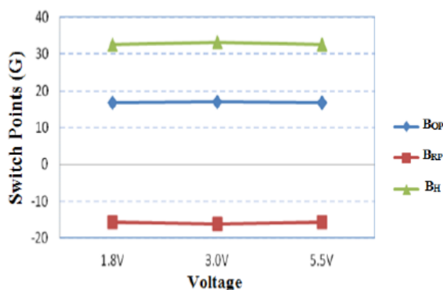
Voltage performance ( T_A=25^\circ C )
